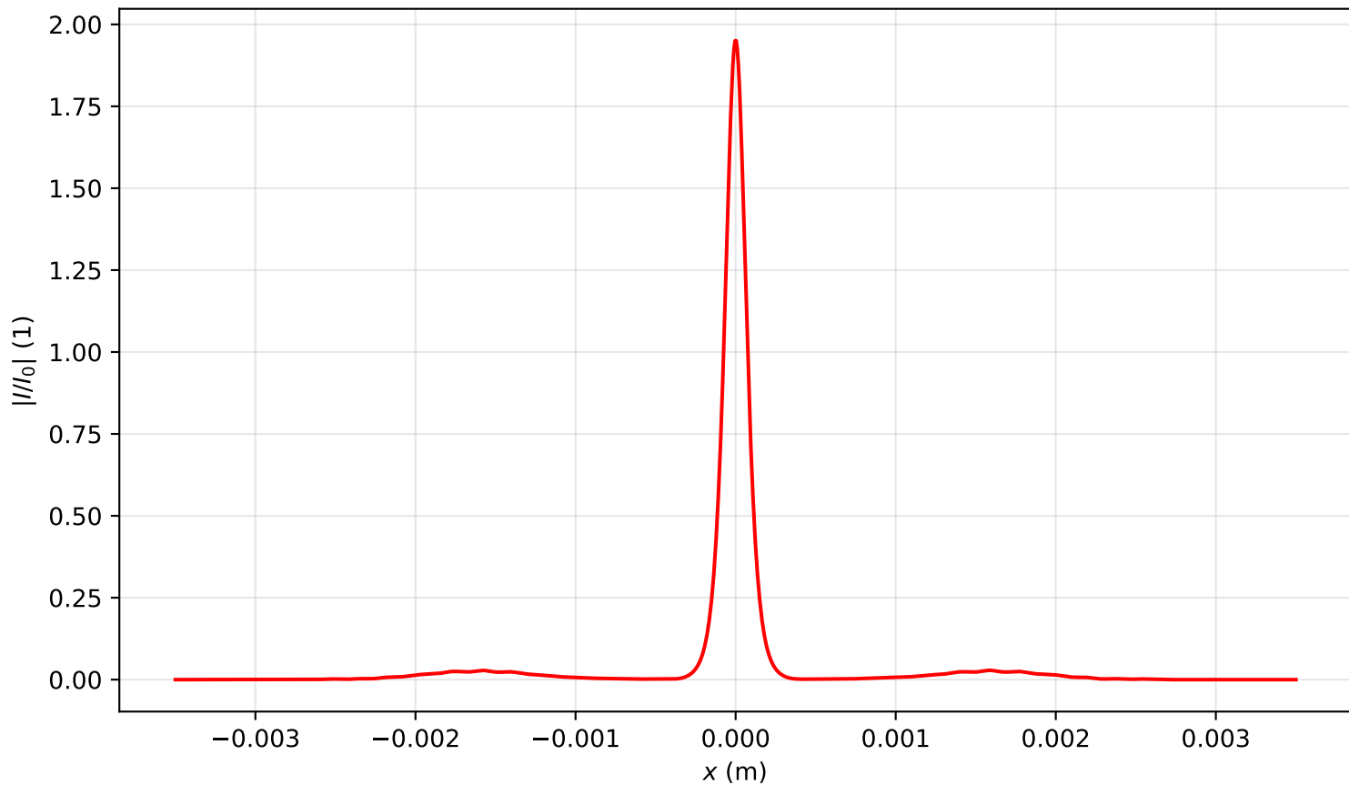
Intensity profile I(x, y = 0, z = 1.274)/I_0 , P_{in}=7.0P_{cr} , artificial time
